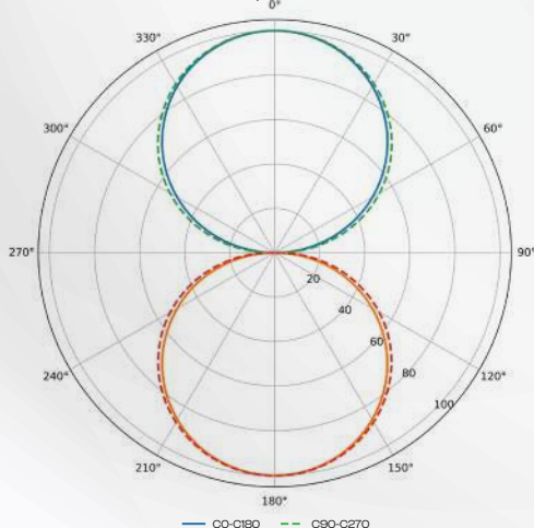
AURL3 Indicative Intensity Distribution Curve Oval Luminaire | Opal PMMA | 120° Beam
