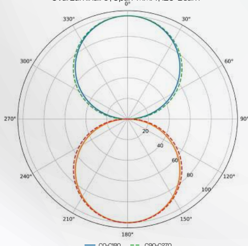
AURLO3 Indicative Intensity Distribution Curve Oval Luminaire | Opal PMMA | 120° Beam
