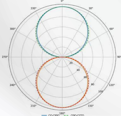
NILE Indicative Intensity Distribution Curve Oval Luminaire | Opal PMMA | 120° Beam
