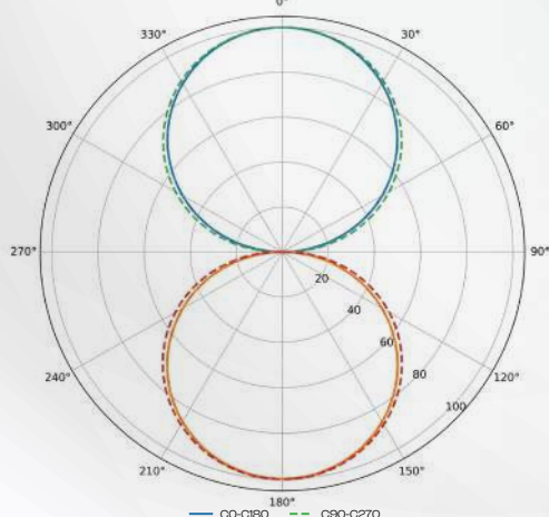
Indicative Intensity Distribution Curve Linear Light 40 mm | Opal PMMA | 120° Beam 0°
